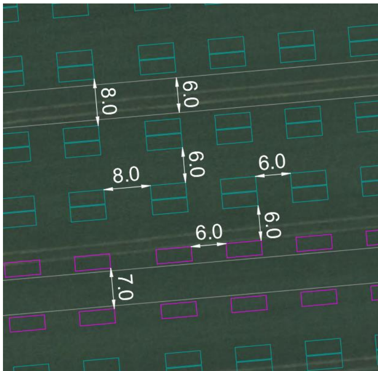
Figure 3.14.1 - BESS and MV Station Unit Spacing
